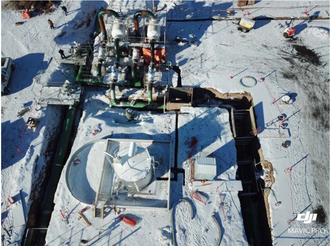
Final connections and tie-ins at the scrubber vessels
