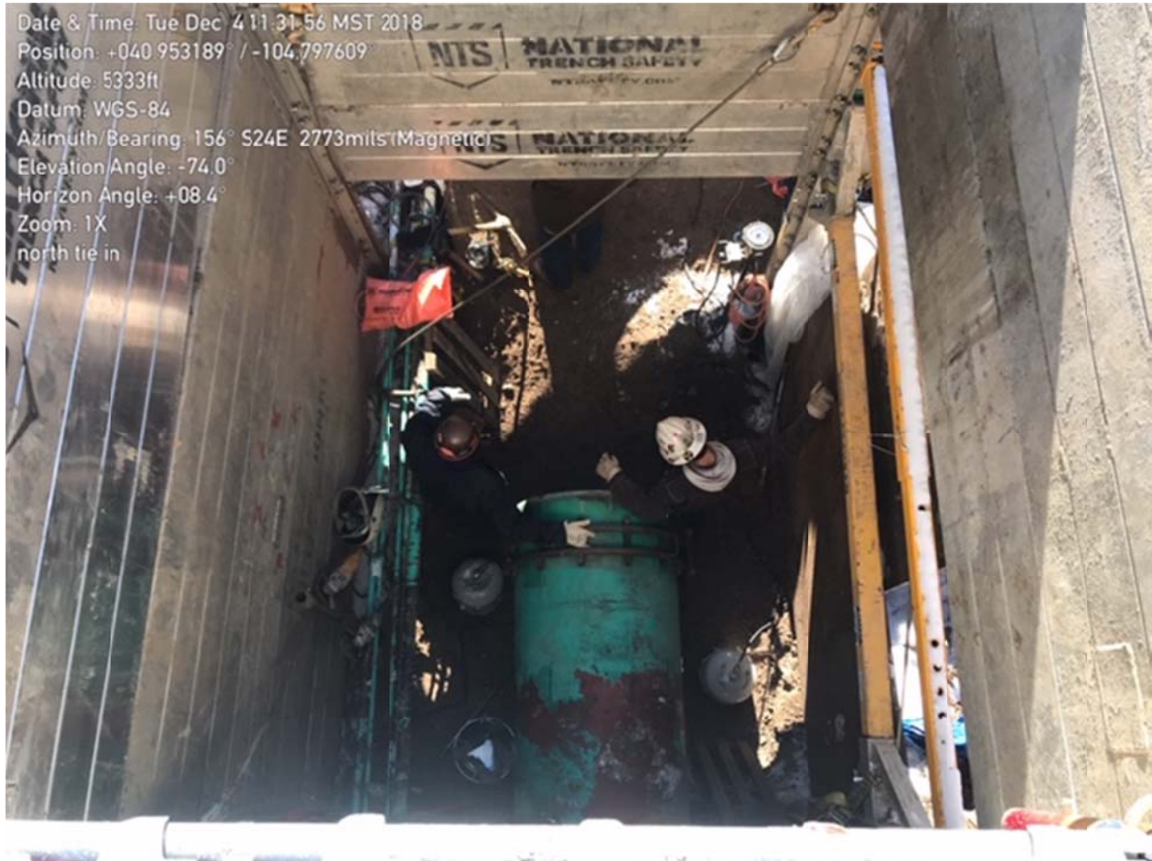
Final pipeline tie-ins
