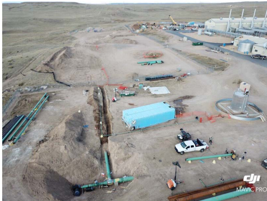
Installation of the 2-inch drain line
